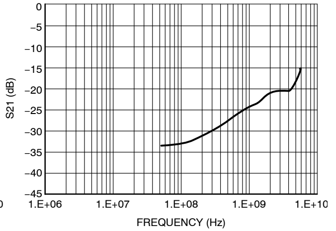
Figure 1. Analog Crosstalk Curve
